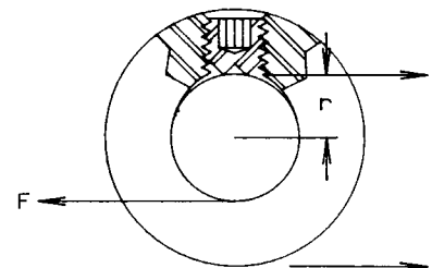
TORSIONAL HOLDING POWER T = Fr
