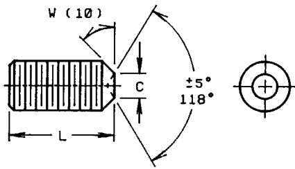
CUP POINT
